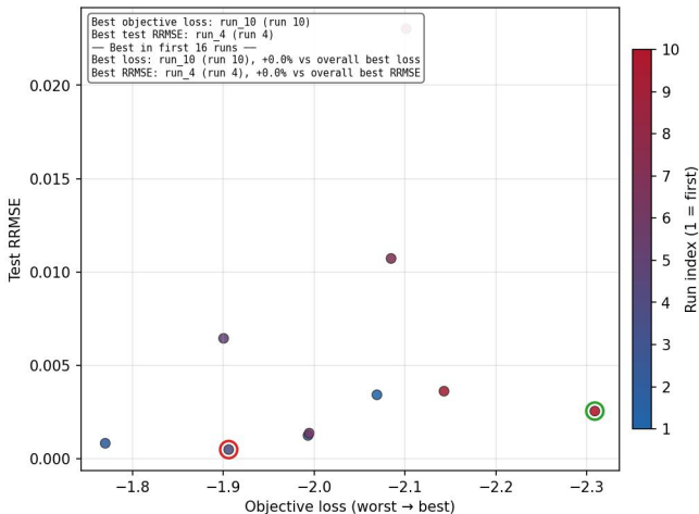
A22_sin_cubic_1Dx_20Dn_[0.0,1.0]_16inits_noiseTest0.0_noiseTrain0.0_x10 Loss vs Test RRMSE
